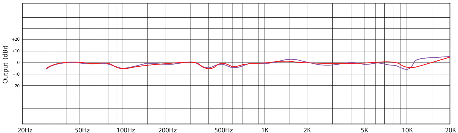
FREQUENCY RESPONSE HR02 FRONT (MONO) & (BACK MONO) @ 1 METRE
