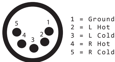
FEMALE 5 PIN
