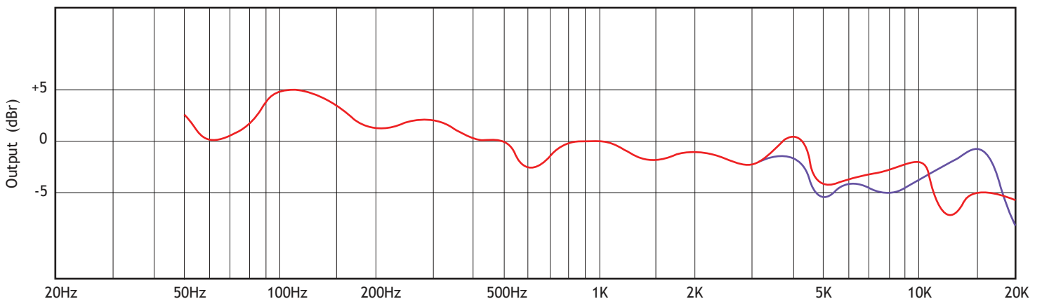
FREQUENCY RESPONSE HRP1 FRONT & BACK
